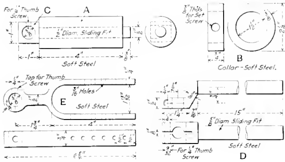
Device for Grinding an Oxy-Acetylene Torch When Cutting on a Circle
